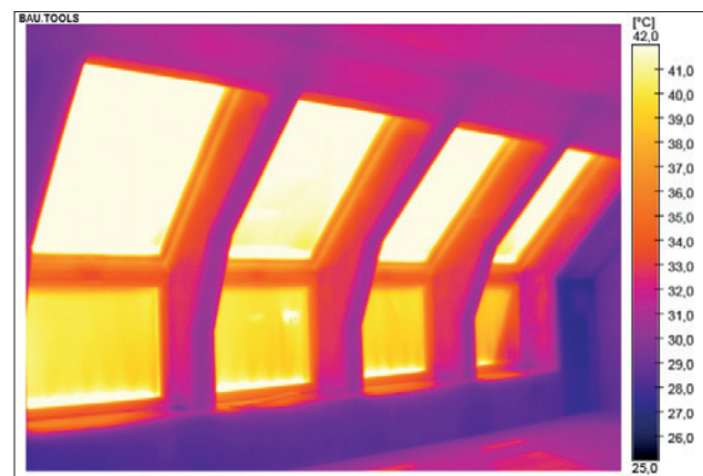
Thermogram "final image" of the recorded sequence. The thermograms do not show any significant differences.
